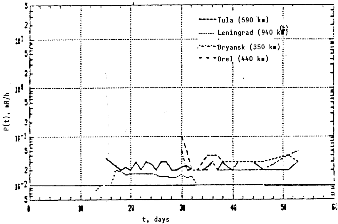
Fig. 72.5. Dynamics of the changes in the gamma dose rates in the open for some regional centres in the Ukrainian SSR (a) and the Russian SFSR (b).
